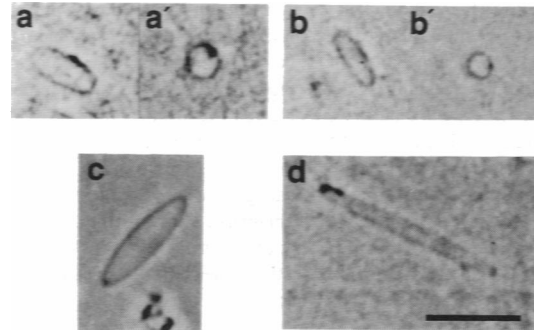
FIGURE 1 Phase-contrast images of four spindle-shaped liposomes, which were taken 15–35 min after the addition of the drug. (a, a', b, b') The images of two liposomes with different view angles demonstrate that they are spindle-shaped. Cytochalasin D concentration was 20 \mu\text{M} . (c) Another spindle-shaped liposome observed at 20 \mu\text{M} cytochalasin D. (d) A spindle-shaped liposome having particularly large axial ratio observed at 100 \mu\text{M} cytochalasin D. This liposome rotated around its long axis, but its width did not change, indicating that it was spindle-shaped. Bar, 10 \mu\text{m} .
