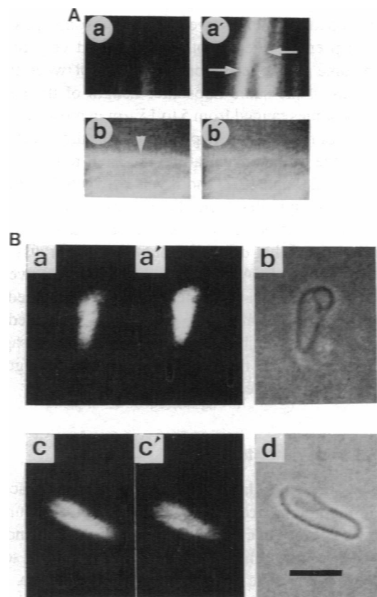
FIGURE 3 (A) Bundles of prodan-actin filaments developed in 20 mM MgCl_2 and observed with fluorescence W-microscope. ( a and a' ) The bundles ( arrows ) are running vertically. ( b and b' ) The bundle runs horizontally ( arrowhead ). ( a and b ) The fluorescence images of vertically polarized fluorescence. ( a' and b' ) The images of horizontally polarized emission. These images indicate that the emission dipole of the actin-bound acrylodan is perpendicular to the axis of an actin filament. Actin concentration was 100 \mu M . (B) Polarized fluorescence and phase-contrast images of two transformed liposomes containing prodan-actin observed in the presence of 50 \mu M cytochalasin D. ( a , a' , and b ) One set of the images. ( c , c' , and d ) The other set. ( a , a' , c , and c' ) Fluorescence images. ( b and d ) Phase-contrast images. ( a and c ) Images of vertically polarized fluorescence. ( a' and c' ) Images of horizontally polarized fluorescence. The liposome in the first set (upper panels) is almost vertical, whereas that in the second set (lower panels) is not completely horizontal. Because of this slight tilt, difference in the intensity of the vertically and horizontally polarized fluorescence in the second set is not as prominent as in the first set. Bar , 10 \mu m .
